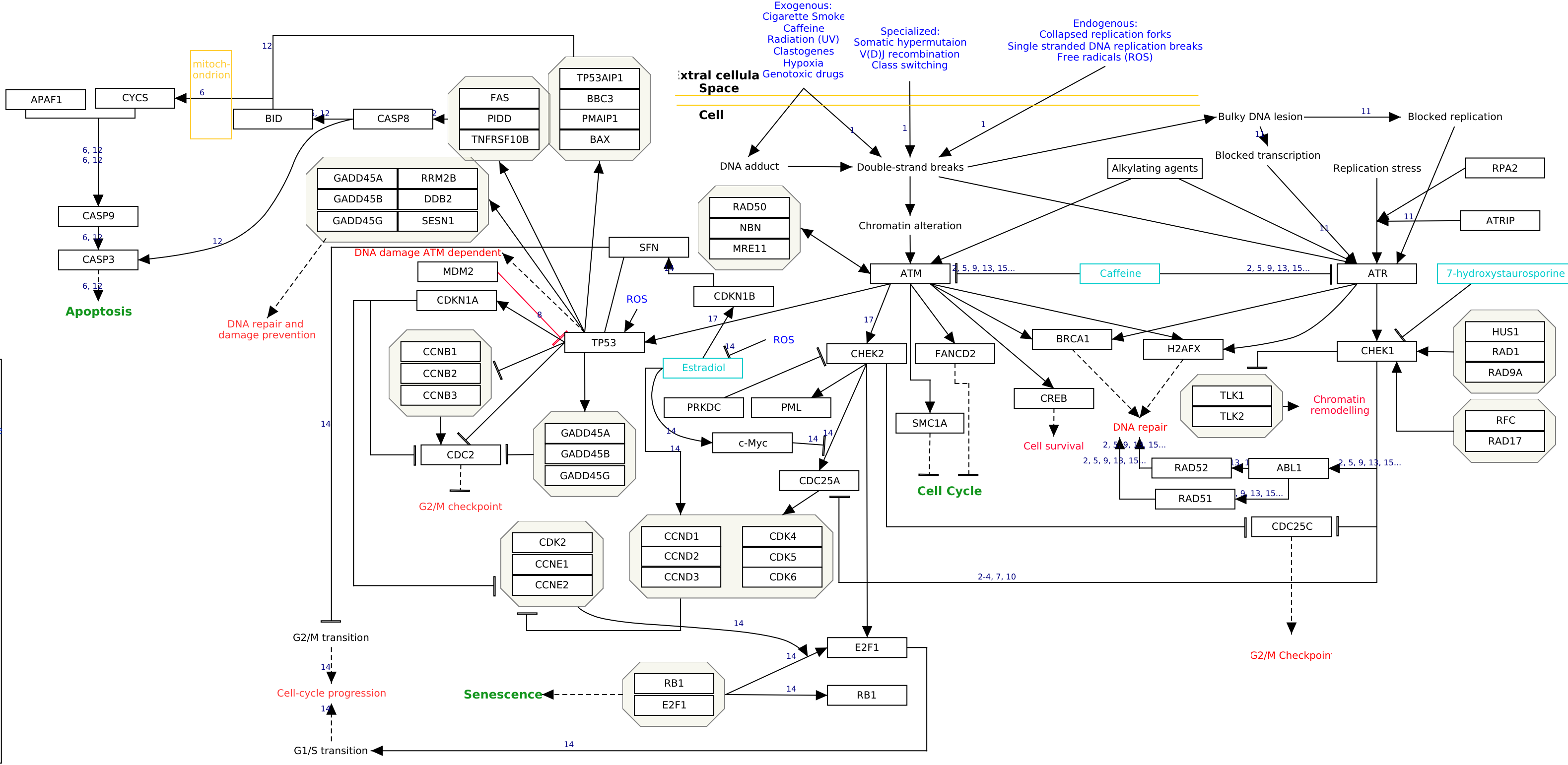
Caption DNA damage source Change in the Cell condition Activation Inhibition Different pathway Gene product Metabolite Membrane
